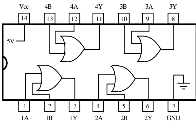
74LS32 Quadrate 2-Input OR Gate
