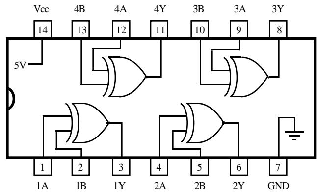
74LS86 Quadrate 2-Input XOR Gate
