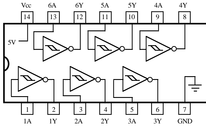
MC14584BCP CD4584 Hex Inverter Schmitt Trigger
