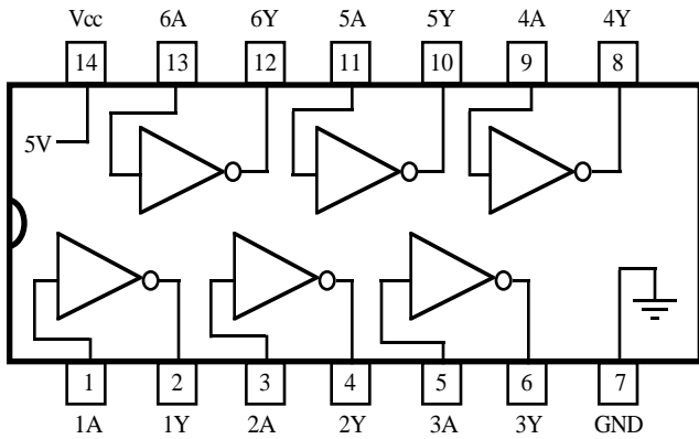
74LS04 Hex Inverter
