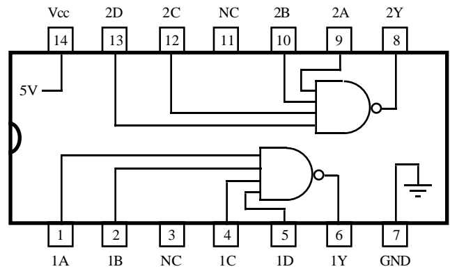
74LS20 Dual 4-Input NAND Gate
