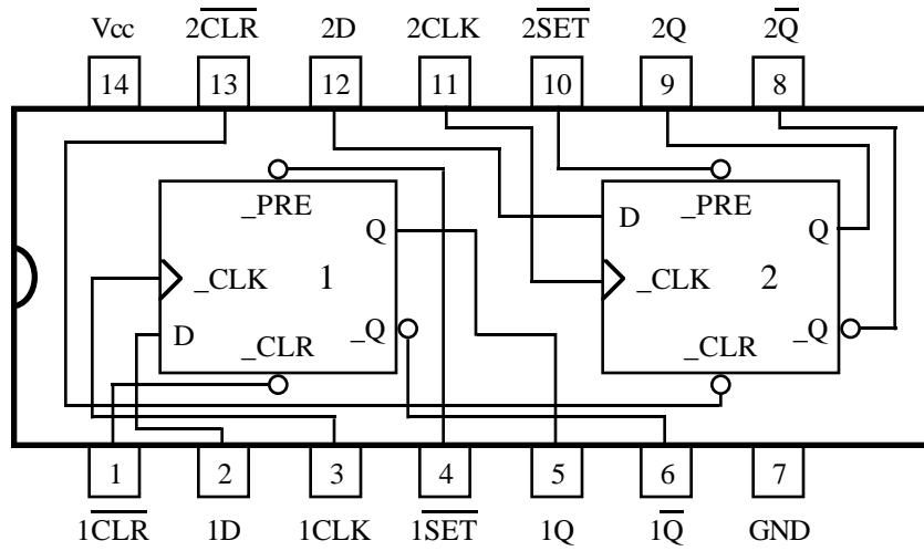
74LS74A Dual D Flip-Flop
