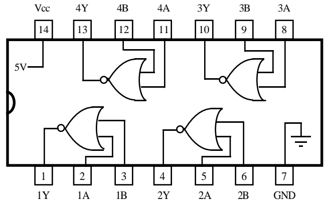
74LS02 Quadrate 2-Input NOR Gate
