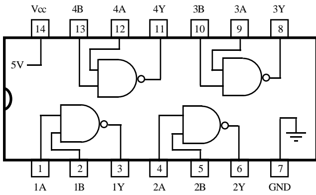
74LS00 Quadrate 2-Input NAND Gate
