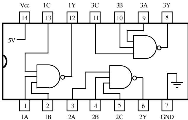
74LS10 Triple 3-Input NAND Gate
