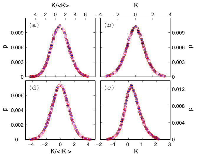
FIG. 7: (Color on-line) Fixed distributions, with circles and crosses showing one renormalization-group transformation and thereby by their exact superposition attesting to the fixed nature of the distributions. The distributions have been binned for exhibition purposes. (a) For the ferromagnetic-spinglass phase boundary, a runaway to infinite coupling; (b) for the paramagnetic-spinglass phase boundary. Both of these fixed distributions are spatially isotropic, attracting isotropic and anisotropic boundaries, and do not obey Nishimori symmetry. (c) For the ferromagnetic-spinglass-paramagnetic multicritical point. This fixed distribution is spatially isotropic and obeys Nishimori symmetry. This fixed distribution attracts the isotropic multicritical point, which obeys Nishimori symmetry, and anisotropic multicritical points, which obey and do not obey Nishimori symmetry. The fixed distributions for the antiferromagnetic-spinglass, columnar-spinglass, layered-spinglass phase boundaries and for the antiferromagnetic-spinglass-paramagnetic, columnar-spinglass-paramagnetic, layered-spinglass-paramagnetic multicritical points are as shown here in (a) and (c) respectively, but with the appropriate K_{xy} \rightarrow -K_{xy} and/or K_z \rightarrow -K_z reflections. (d) Fixed distribution for the spin-glass phase. This phase sink is an isotropic runaway, attracting both spatially isotropic and anisotropic spin-glass phase points, and does not obey Nishimori symmetry.
