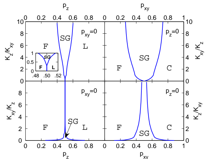
FIG. 4: (Color on-line) Zero-temperature phase diagrams of the longitudinal (left column) and transverse (right column) spin-glass systems. With the appropriate reversal in variables, the transverse and longitudinal spin-glass phase diagrams are seen here to be qualitatively similar, but quantitatively different. The spin-glass phase is more extensive in the transverse case. All phase transitions in this figure are second order.
