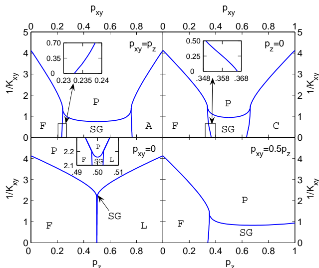
FIG. 3: (Color on-line) Temperature-concentration phase diagrams for isotropically mixed (upper left), transverse (upper right), longitudinal (lower left), and p_{xy} = 0.5p_z spin-glass systems. In all cases, K^z/K^{xy} = 0.5 . The upper left and right phase diagrams are seen to be, respectively, reentrant and forward, namely with a ferromagnetic phase that, respectively, recedes from or proceeds towards the spin-glass phase as temperature is lowered, as clearly seen in the insets. There are no points obeying Nishimori symmetry in the phase diagrams of this figure. Note the remarkably narrow spin-glass phase, reaching zero-temperature, in the longitudinal spin-glass system, as also seen in the inset. All phase transitions in this figure are second order.
