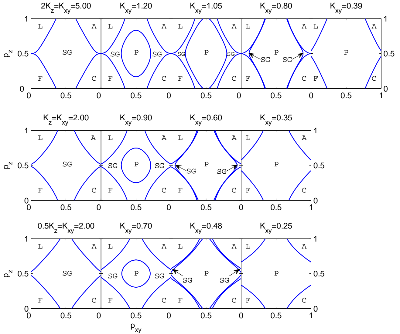
FIG. 1: (Color on-line) Top line: Constant-temperature cross-sections of the global phase diagram for K^z/K^{xy} = 0.5 , as a function of p_{xy} and p_z , which are the concentrations of antiferromagnetic xy and z bonds, respectively. At low temperatures (high K^{xy} ), the central spin-glass (SG) phase separates the corner ferromagnetic (F), columnar (C), antiferromagnetic (A), and layered (L) phases. As temperature increases, the paramagnetic (P) phase appears at the central point, first reaches the transverse spin-glass system and eliminates the spin-glass phase, then reaches the longitudinal spin-glass system and eliminates the spin-glass phase. In the latter system, the spin-glass and paramagnetic phases simultaneously occur for a very narrow range of temperatures, as also seen in the inset in the lower left panel of Fig.3. Middle line: Constant-temperature cross-sections for K^z = K^{xy} . Bottom line: Constant-temperature cross-sections for K^z/K^{xy} = 2 . All phase transitions in this figure are second order.
