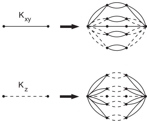
FIG. 2: Construction of the uniaxially anisotropic d=3 hierarchical model. Two graphs are mutually and repeatedly self-imbedded. Note that for K^{xy} = 0, K^z = 0 , and K^{xy} = K^z , the system reduces respectively to the d = 1 , isotropic d = 2 and d = 3 systems.
