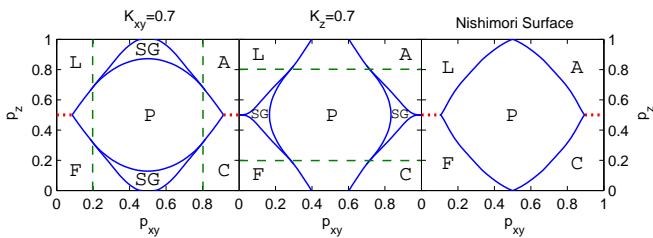
FIG. 6: (Color on-line) The Nishimori condition for K_z is held throughout the leftmost figure and for K_{xy} throughout the center figure. The complimentary Nishimori condition, for K_{xy} and K_z respectively, is held along the dashed straight lines, which intersect the ordered (F, L, A, or C)-spinglass-paramagnetic multicritical points. In the rightmost figure both conditions are satisfied throughout the figure. In this figure, the phase boundaries around the paramagnetic phase are actually lines of the multicritical points where the paramagnetic, ordered (F, L, A, or C), and spin-glass (not seen in this cross-section) phases meet. In the side figures, first-order boundaries (dotted) occur between the ferromagnetic and layered phases, and between the antiferromagnetic and columnar phases, terminating at d = 2 critical points. All other phase transitions (full lines) in this figure are second order.
