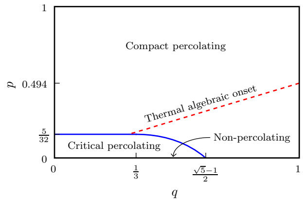
FIG. 4: (Color online) Geometric phase diagram of the network with short-range and long-range random bonds, exhibiting compact percolating, critical percolating, and non-percolating phases. The dashed line indicates the onset of high-temperature algebraic order in an Ising magnetic model on this network. It is thus seen that this thermal onset has no signature in the geometric correlations.
