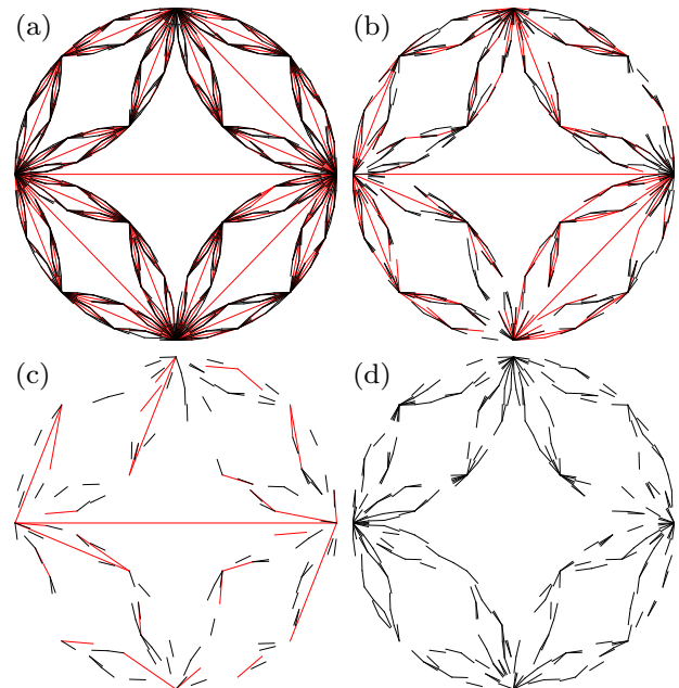
FIG. 2: (Color online) Different realizations of the random network: (a) In the compact percolating phase, with q = p = 0.8 . (b) In the compact percolating phase, with q = p = 0.4 . (c) In the algebraic percolating phase, with q = p = 0.1 . (d) In the non-percolating phase, with q = 0.3, p = 0 .
