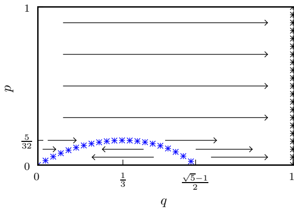
FIG. 3: (Color online) Renormalization-group flow diagram of percolation on the network with short-range and long-range random bonds.
