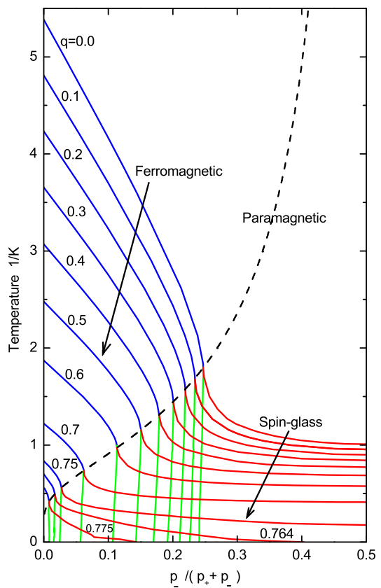
FIG. 2: (Color on-line) Calculated phase diagrams at constant quenched dilution q = 1 - p_+ + p_- . The phase diagrams being symmetric about p_-(p_+ + p_-) = 0.5 , with the anti-ferromagnetic phase replacing the ferromagnetic phase, only the p_-(p_+ + p_-) < 0.5 halves are shown. All phase transitions (full lines) are second order. The dashed curve is the Nishimori symmetry line given by Eq.(2). All multicritical points, mediating the ferromagnetic, spin-glass, and paramagnetic phases, lie on the Nishimori symmetry line.
