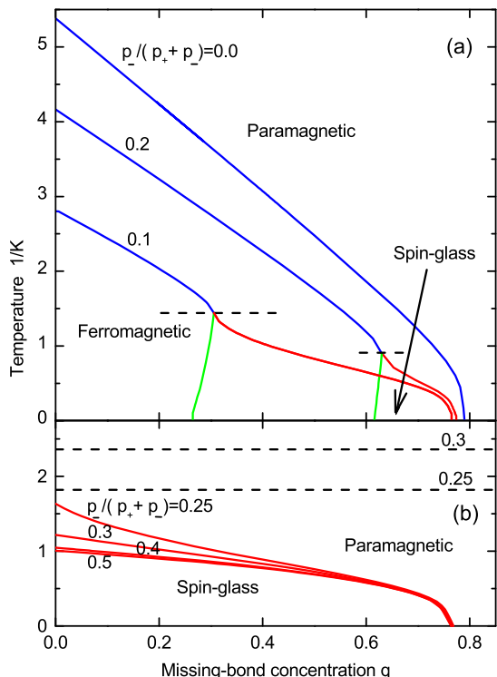
FIG. 1: (Color on-line) Calculated phase diagrams at constant p_-(p_+ + p_-) . All phase transitions (full lines) are second order. The dashed horizontal lines (shown only partly in (a)) are not phase boundaries, but the Nishimori symmetry lines, given by Eq.(2), for each value of p_-(p_+ + p_-) . The multicritical points in (a), mediating the ferromagnetic, spin-glass, and paramagnetic phases, occur on the Nishimori symmetry lines. These lines do not cross the phase boundaries at any other type of point. Thus, the Nishimori symmetry lines in (b) are at temperatures above the phase boundaries.
