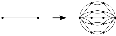
FIG. 4: The d = 3 hierarchical lattice for which our calculation is exact is constructed by the repeated imbedding of the graph as shown in this figure. This hierarchical lattice gives accurate results for the critical temperatures of the d = 3 isotropic and anisotropic Ising models on the cubic lattice [6].
