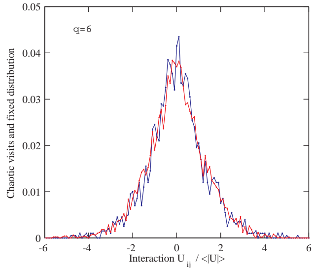
FIG. 6: (Color online) Comparison, showing the coincidence, of the chaotic visits of the consecutively renormalized interactions at a given position of the system (for 2,000 renormalization-group iterations) and of the asymptotic distribution of the interactions across the system at a given renormalization-group step, for the spin-glass phase. The Lyapunov exponent is \lambda = 1.93 . Identical asymptotic behavior occurs for all q -state clock spin-glass phases, as shown in Fig.5. The divergence of \langle |U| \rangle is as b^{0.24n} , where n is the number of iterations.
