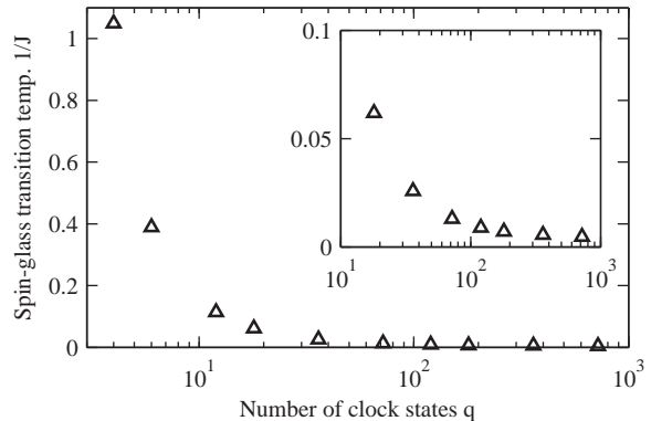
FIG. 4: The calculated transition temperatures between the spin-glass phase and the paramagnetic phase, at p = 0.5 , as a function of q , up to very large values of q = 720 . Note the logarithmic scale of the horizontal axes. The slow decay of the transition temperature suggests that a zero-temperature spin-glass phase exists in the ( q \rightarrow \infty ) XY model limit.
