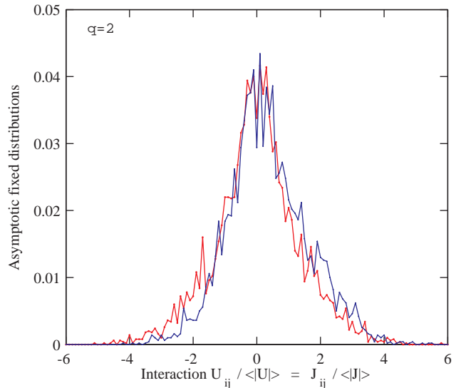
FIG. 8: (Color online) Two different, non-coinciding strong-coupling fixed distributions: The fixed distribution and, equivalently, chaotic renormalization-group trajectory onto which the spinglass-ferromagnetic phase boundary of the q = 2 -state model in d = 3 renormalizes. For comparison and distinction, the asymptotic fixed distribution and chaotic renormalization-group trajectory of the corresponding spin-glass phase is also shown. The latter curve is symmetric around U_{ij} / \langle |U| \rangle = 0 , whereas the former curve is noticeably displaced towards positive (ferromagnetic) interaction values. Note that these are strong-coupling distributions and are therefore shown as a fraction of the diverging \langle |U| \rangle . The divergence of \langle |U| \rangle is as b^{0.46n} and b^{0.24n} , where n is the number of iterations, respectively for the phase boundary and phase sink cases. Thus, even small shifts in the shown curves signify large differences in the interaction values. The Lyapunov exponents are \lambda = 1.69 and 1.93 , respectively for the phase boundary and phase sink cases. For q = 2 , the form of the interaction in Eq.(1) is conserved under renormalization, which is reflected in the horizontal axis label here.
