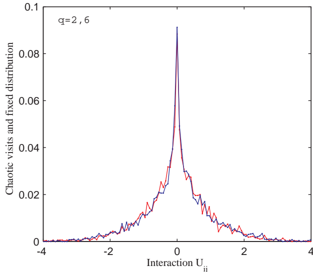
FIG. 7: (Color online) The fixed distribution and, equivalently, chaotic renormalization-group trajectory onto which the phase boundary between the spin-glass and paramagnetic phases renormalizes, for the q = 2 and q = 6 -state clock models in d = 3 . The Lyapunov exponent is \lambda = 1.35 . Identical asymptotic behavior occurs for all q . Note that the chaotic behavior and fixed distribution are at intermediate coupling strength, with \langle |U| \rangle = 0.686 for all q .
