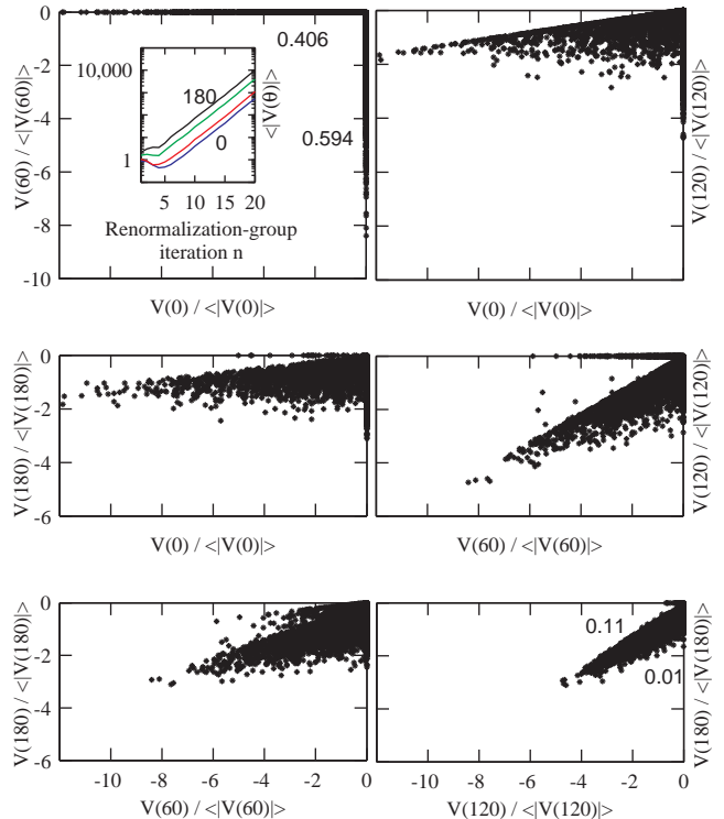
FIG. 9: The fixed distribution and, equivalently, chaotic renormalization-group trajectory onto which the spinglass-ferromagnetic phase boundary of the q = 6 -state clock model in d = 3 renormalizes. The coupled distributions of the interactions V(\theta) / \langle |V(\theta)| \rangle are shown, while next to each axis, the fraction of points on the axis are given. The full fixed distribution has the form P(\{V(0), V(60), V(120), V(180)\}) , as a coupled function of its arguments. This is a strong-coupling behavior: The inset in the upper left panel shows, with the logarithmic vertical scale, the diverging \langle |V(\theta)| \rangle as a function of renormalization-group iteration n , the consecutive curves being for \theta = 180, 120, 60, 0 . It is seen that, for all \theta , \langle |V(\theta)| \rangle diverges as b^{0.46n} , where n is the number of iterations.
