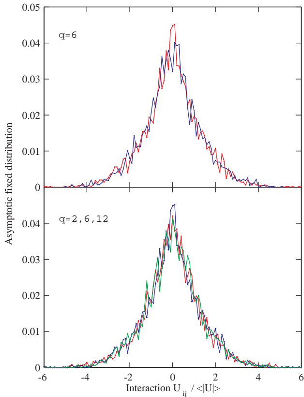
FIG. 5: (Color online) Asymptotic fixed distribution, under renormalization-group transformations, of the interactions in the spin-glass phase, namely the renormalization-group sink of the spin-glass phase. Note that these are strong-coupling distributions, as the average interaction strength \langle |U| \rangle diverges to infinity under the renormalization-group transformations. The divergence of \langle |U| \rangle is as b^{0.24n} , where n is the number of iterations. Top: For the q = 6 -state clock model in d = 3 , for a trajectory starting in the spin-glass phase at p = 0.5 and temperature 1/J = 0.05 , the distributions after 20 and 21 renormalization-group steps are shown. It is seen that these two distributions coincide, signifying a fixed distribution. Bottom: Asymptotic fixed distributions of the spin-glass phases for the q = 2 (Ising), 6, 12-state clock models in d = 3 . These distributions are reached after 20 renormalization-group steps, starting at p = 0.5 and temperature 1/J = 0.05 . Note that the spin-glass sink fixed distributions for different values of q coincide. The Lyapunov exponent is \lambda = 1.93 for the single, universal distribution that is illustrated in this figure.
