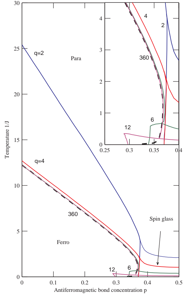
FIG. 2: (Color online) Calculated phase diagrams of the q = 2, 4, 6, 12 clock spin-glass models in d = 3 dimensions. The phase diagram for the XY limit, namely q \rightarrow \infty , is also shown, by the dashed curve, calculated here with q = 360 clock states. As q is increased, it is found that the spin-glass phase retreats to lower temperatures while further protruding into the ferromagnetic phase. In the XY limit, the spin-glass phase disappears at zero temperature (see Fig. 4 below), as the phase boundary between the remaining ferromagnetic and paramagnetic phases numerically stabilizes, on the scale of the figure, for q \gtrsim 6 .
