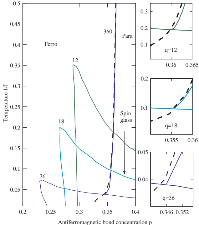
FIG. 3: (Color online) Phase diagrams of the q = 12, 18, 36 clock spin-glass models in d = 3 dimensions. Two new phenomena are simultaneously detected here: (1) double reentrance: paramagnetic-ferromagnetic-spin-glass-ferromagnetic as temperature is lowered, (2) lateral reentrance: ferromagnetic-spin-glass-ferromagnetic-paramagnetic as p is increased. The XY limit is given, calculated here with q = 360 clock states, by the dashed curve. The panels on the right show the region of the multicritical point, where the three phase boundary lines meet, for each q case along with the ferromagnetic-paramagnetic phase boundary of the XY limit.
